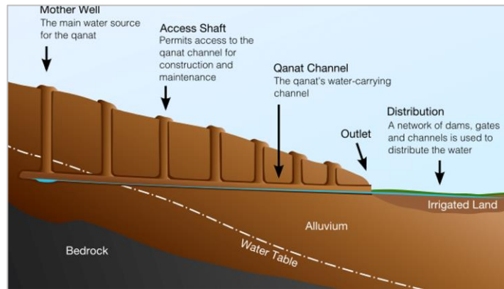
Figure 4: The Irrigation System of Qanat
