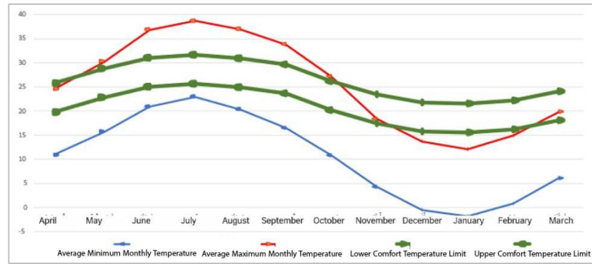
Figure 9: Monthly temperature conditions relative to the comfort range. (Authors).
