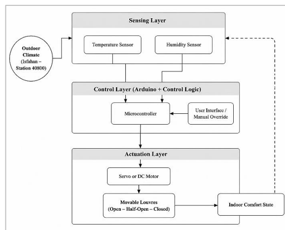
Figure 10: Conceptual control architecture of the interactive envelope, showing the sensor–controller–motor loop validated through the 1:20 functional prototype. ( Authors ).
