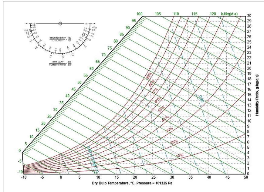
Figure 3: Relationship between temperature, humidity ratio, and relative humidity on the psychrometric chart. (flycarpet.net).
