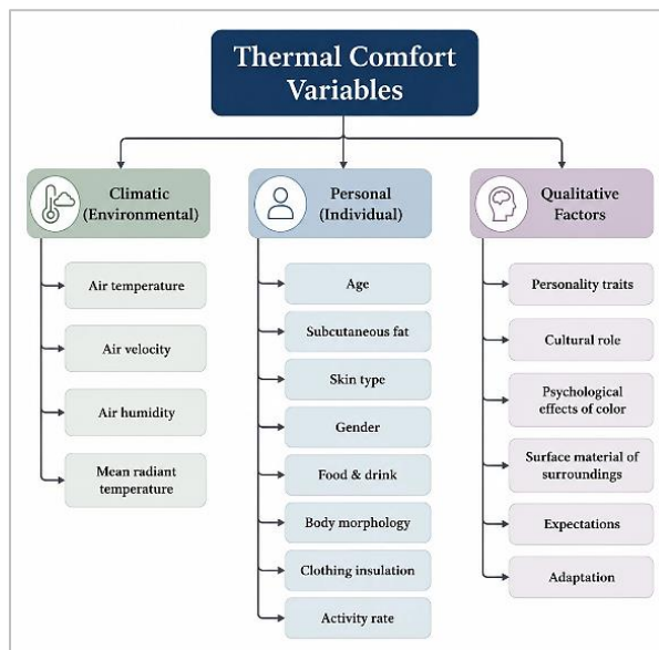
Figure 2: Thermal comfort and its interactions with quantitative and qualitative factors, adapted from (Mortaheb, 2022).
