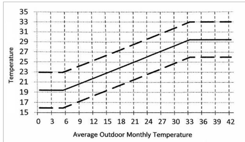
Figure 4: Acceptable thermal comfort temperature for the population of Iran. (Heydari, 2014).
